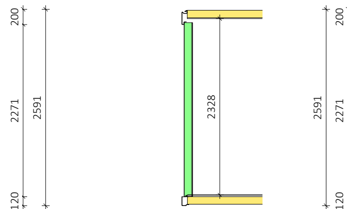
Interior Height 1 : 50
