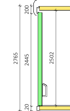
Interior Height 1:50
