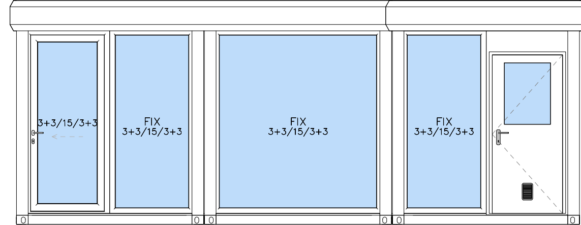
View Right side 1:50
