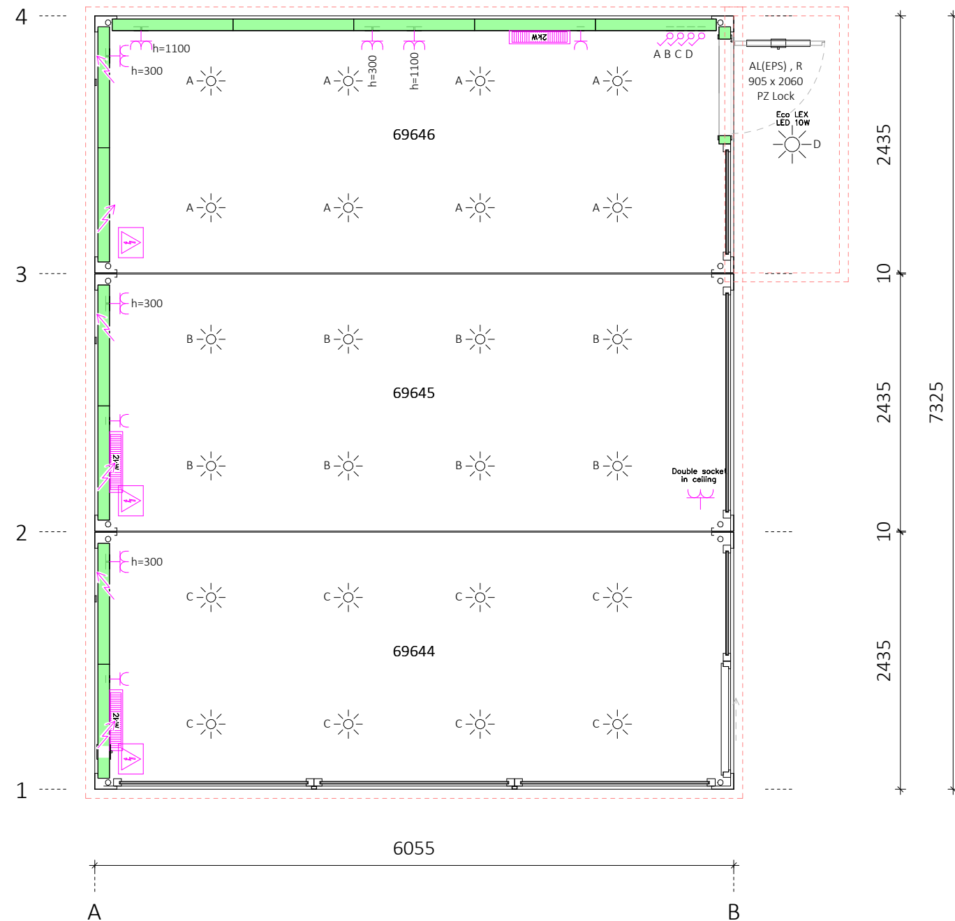
Floor Plan 1:50
